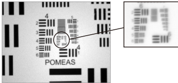
Ordinary zoom lens 5× resolution board
